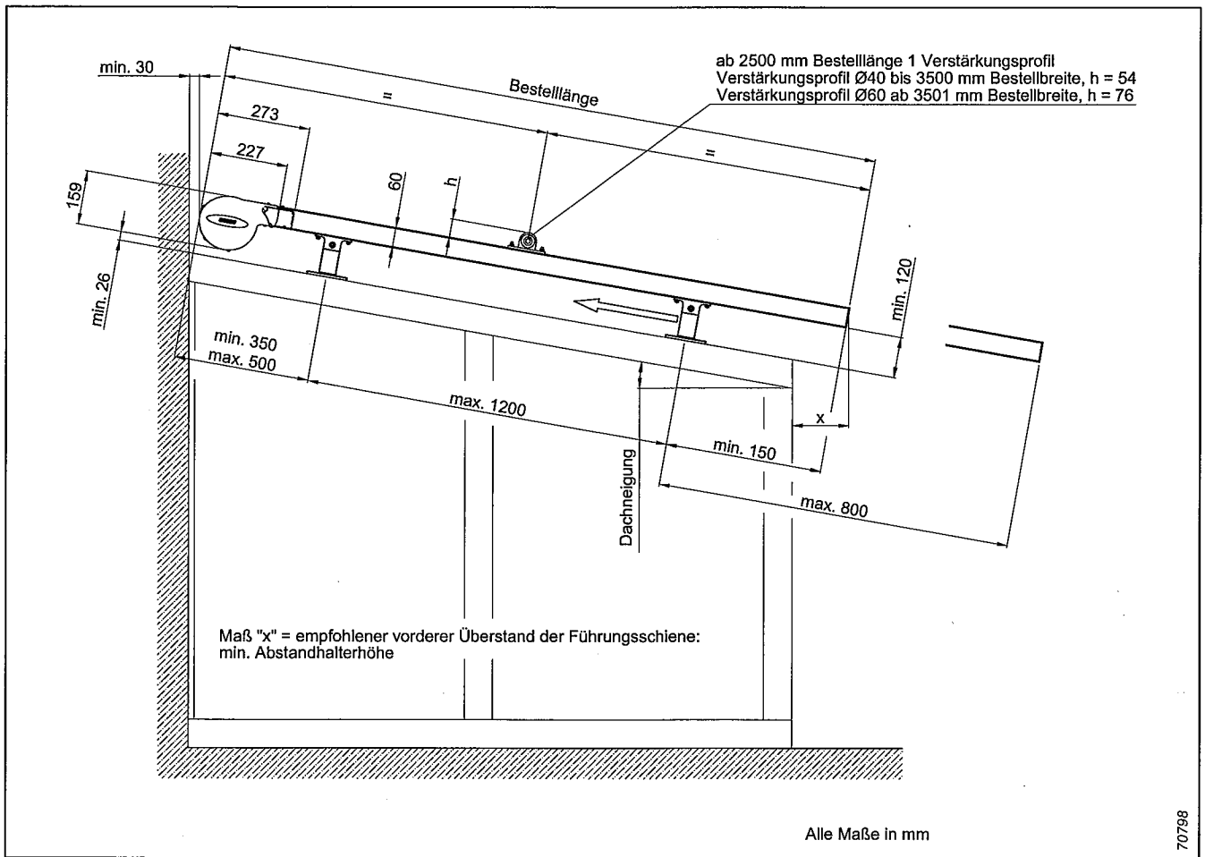
Abb. 326: Wintergarten-Markise W20
